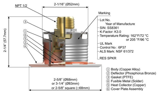
Figure 1: Model RC-RES K = 3.0
